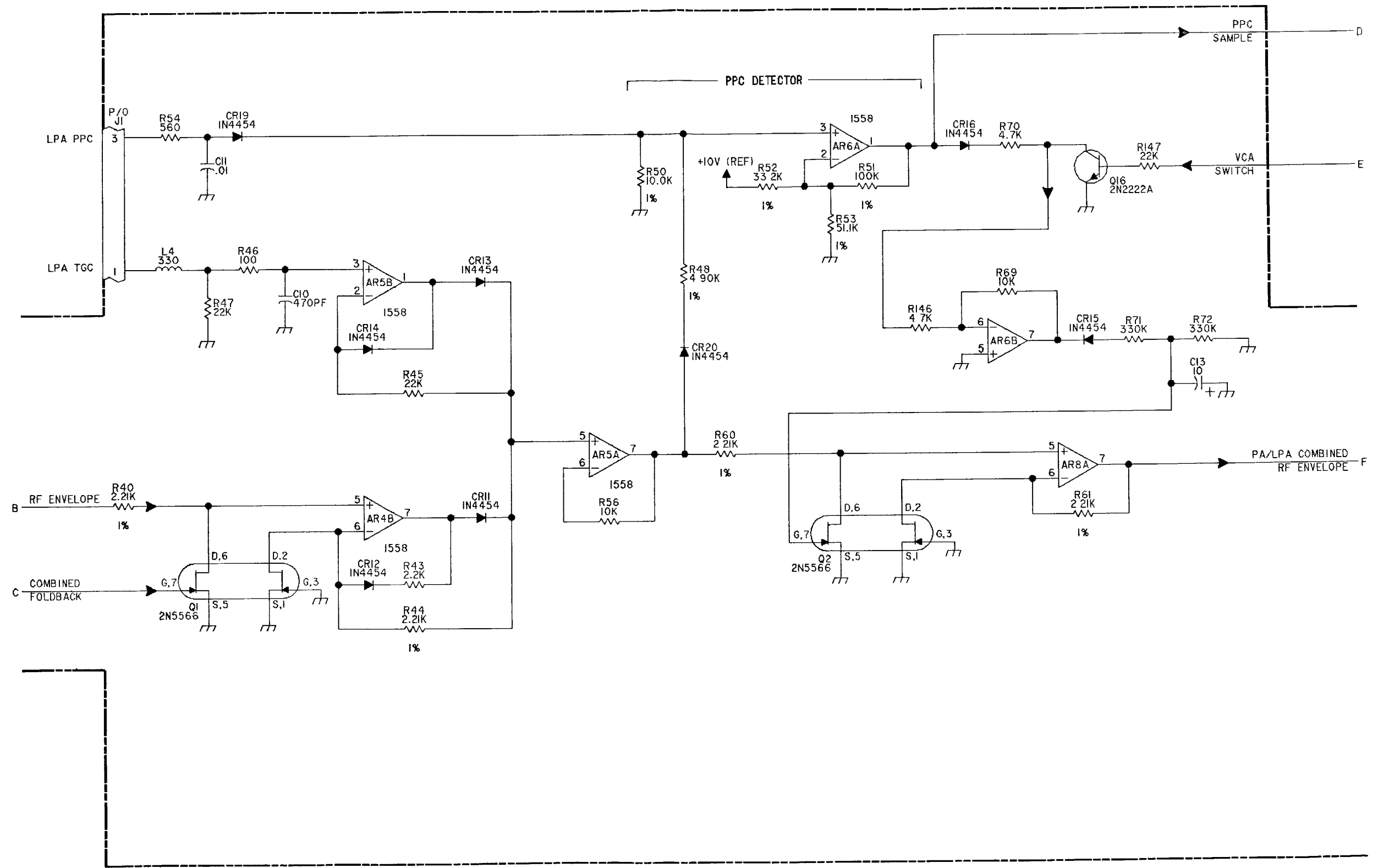
FO-8. AGC/TGC PWB ASSY, A1A6 (Sheet 5 of 9)
