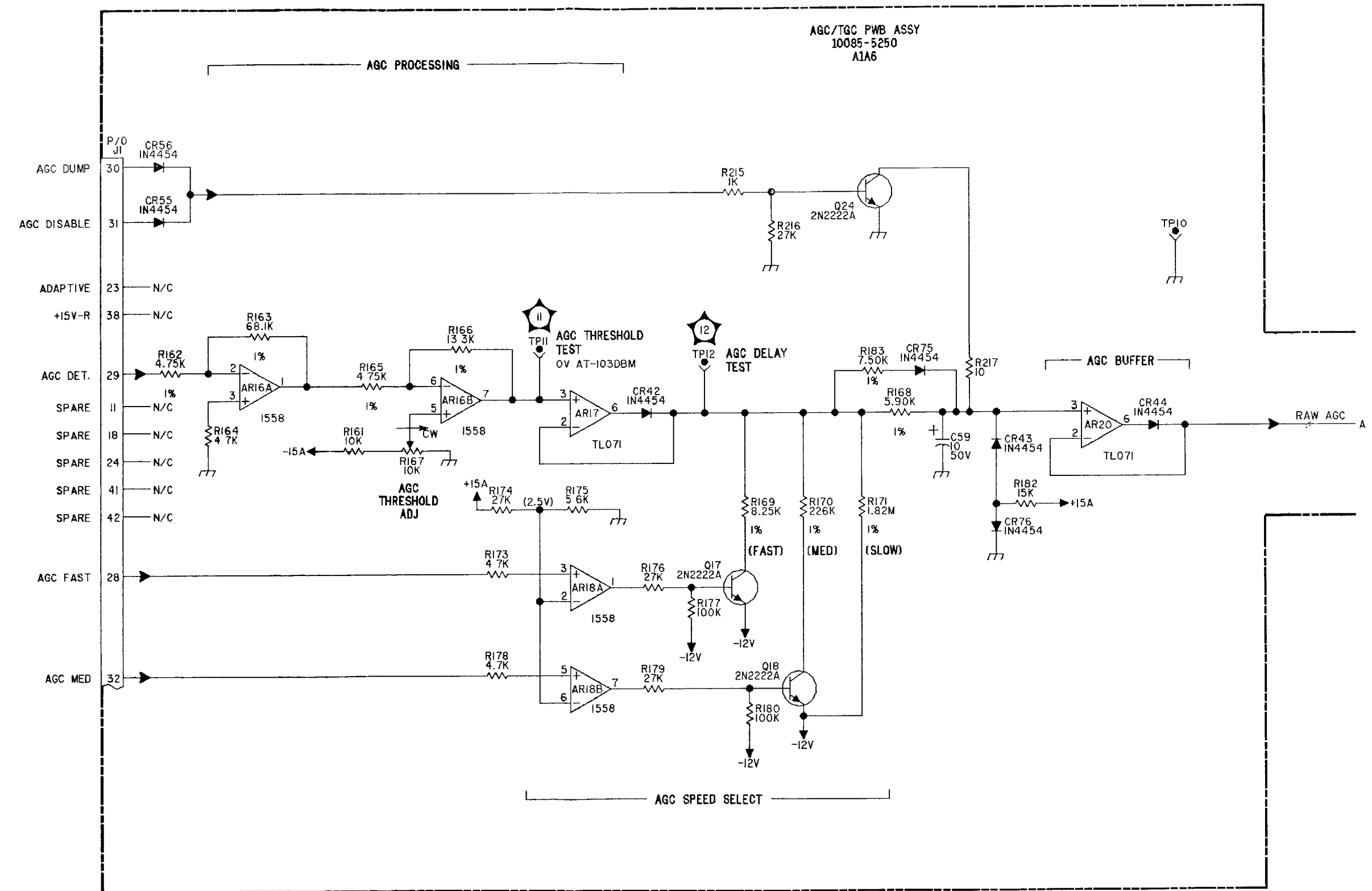
FO-8. AGC/TGC PWB ASSY, A1A6 (Sheet 1 of 9)
